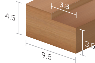
Frame 2"x 4"
